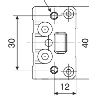
M4 (depth 6) (n°2 Flange fixing threads)
