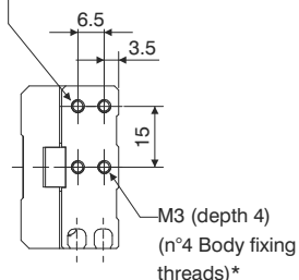
Mounting surface for stroke regulation block
